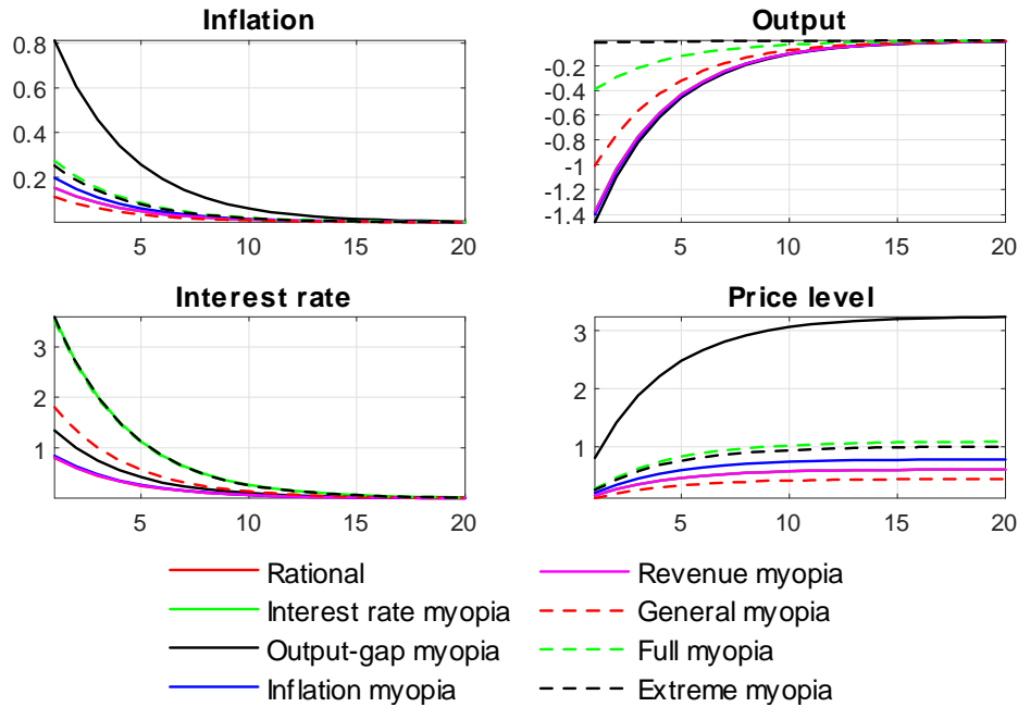
Figure 12. Discretion: Robustness.
