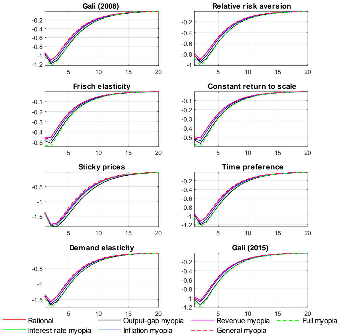
Figure 4. Commitment: Output.
