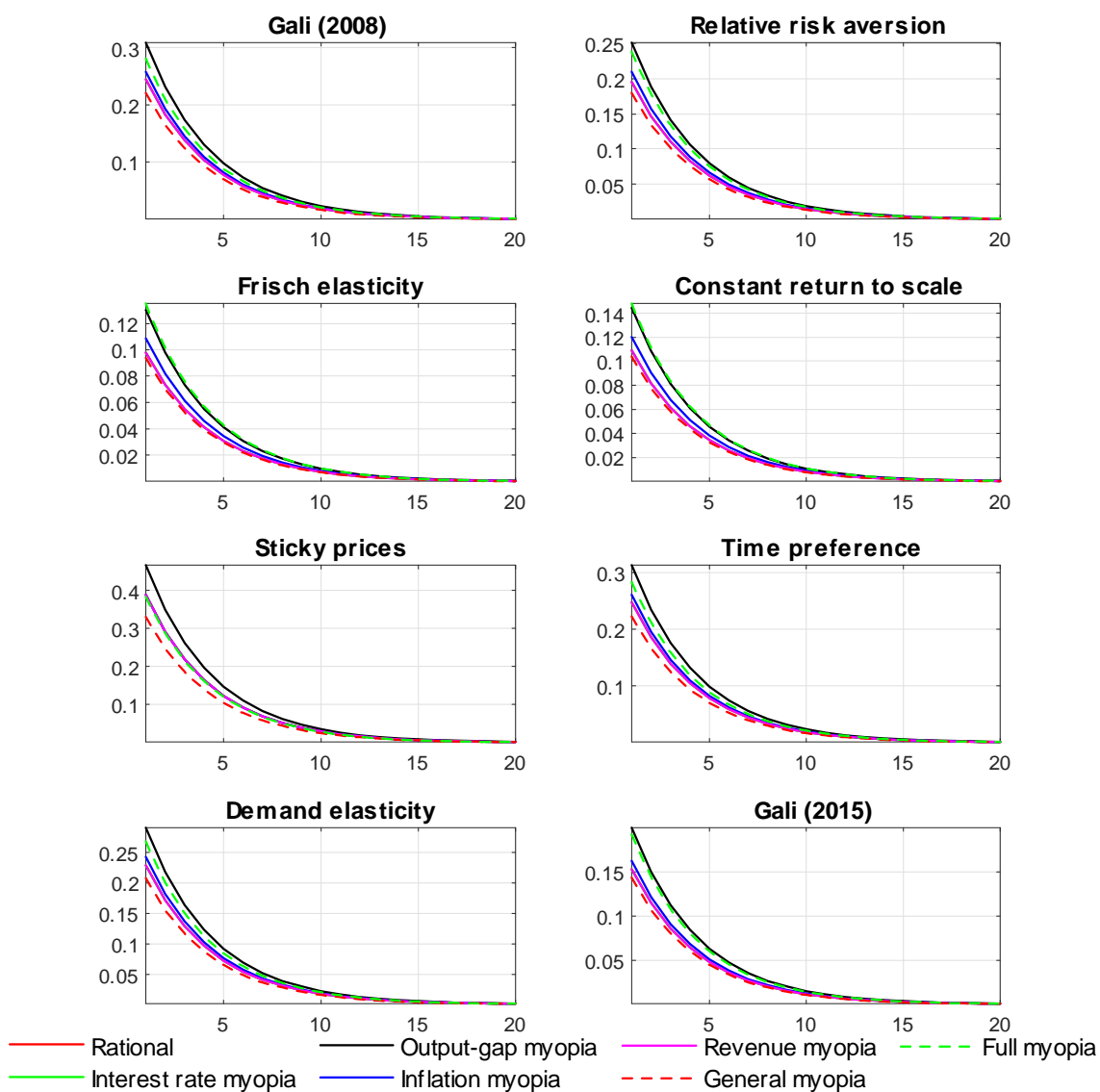
Figure 7. Discretion: Inflation.
