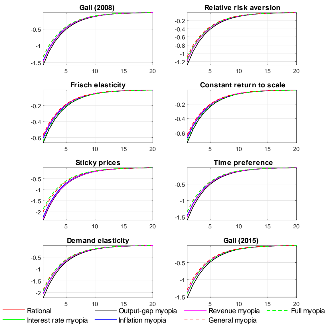
Figure 8. Discretion: Output.
