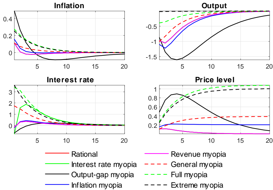
Figure 11. Commitment: Robustness.
