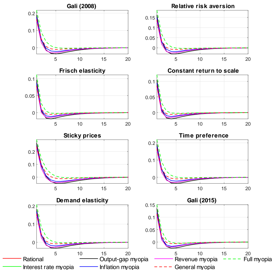
Figure 3. Commitment: Inflation.
